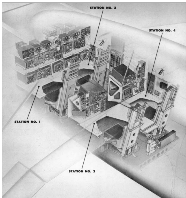
RB-66C aft ECM compartment showing EWO stations. (From Mick Roth & Rene Francillon, Douglas B-66, Aerofax Minigraph 19, via the author)
