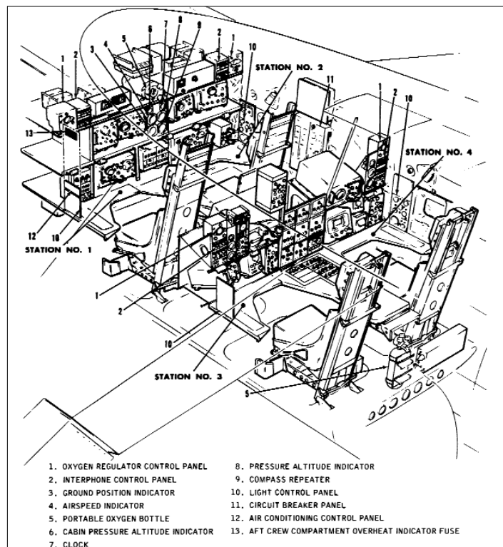
The RB-66C designation was changed to EB-66C and shows slight difference in equipment in this 1970 configuration. (From Mick Roth & Rene Francillon, Douglas B-66, Aerofax Minigraph 19, via the author)
