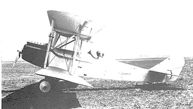
Curtiss "Night Mail" (Curtiss Wright #T2503)
