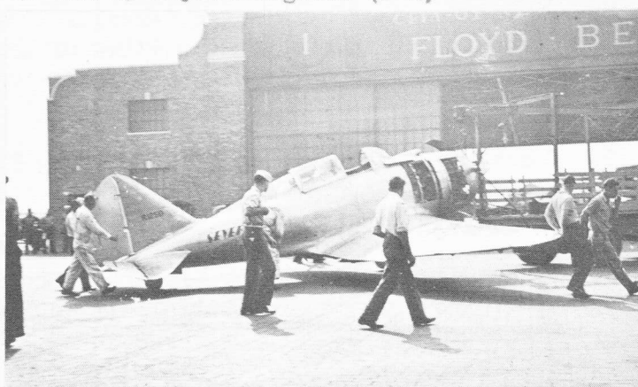
6. AP-2 after ground-loop
