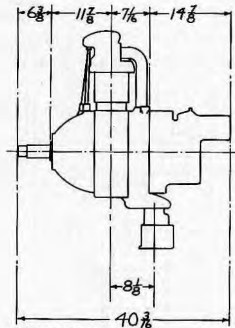
JACOBS AIRCRAFT ENGINE COMPANY Pottstown, Penna. JACOBS MODEL L-4M — 225 H.P. 7 CYLINDER RADIAL AIRCOOLED
