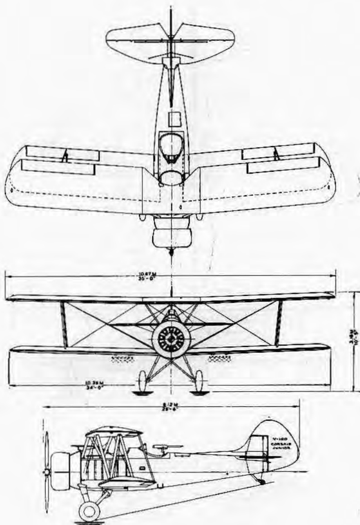
CHANCE VUGHT CORPORATION East Hartford, Conn. CORSAIR JUNIOR V-100 — 2 PLACE ENGINE: PRATT & WHITNEY WASP JUNIOR
