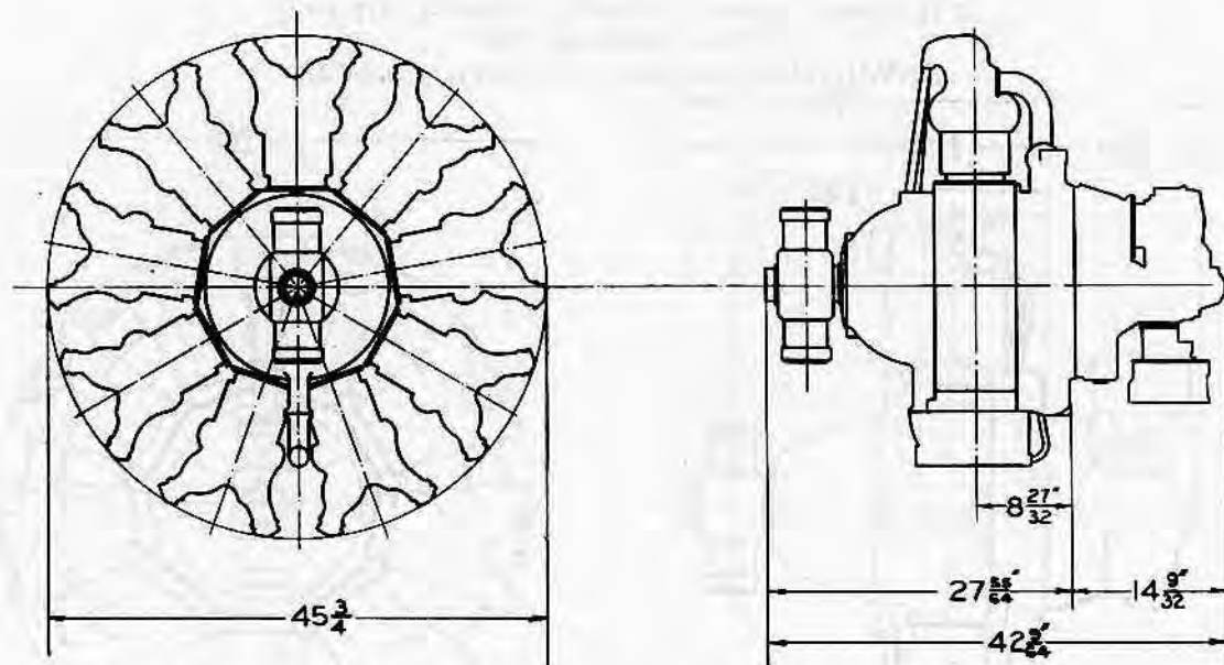
PRATT & WHITNEY AIRCRAFT COMPANY East Hartford, Conn. WASP JUNIOR B — 320-420 H.P. 9 CYLINDER RADIAL AIRCOOLED
