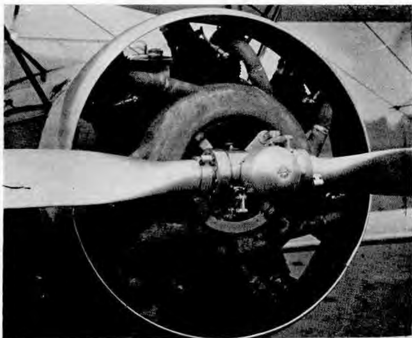
ECLIPSE VARIABLE PROPELLER HUB
