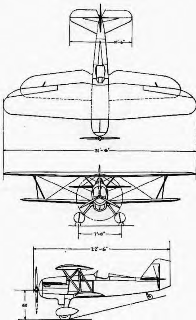
CURTISS AEROPLANE & MOTOR COMPANY Buffalo, N. Y. HAWK PURSUIT P 6-E ENGINE: CURTISS CONQUEROR 675 H.P.
