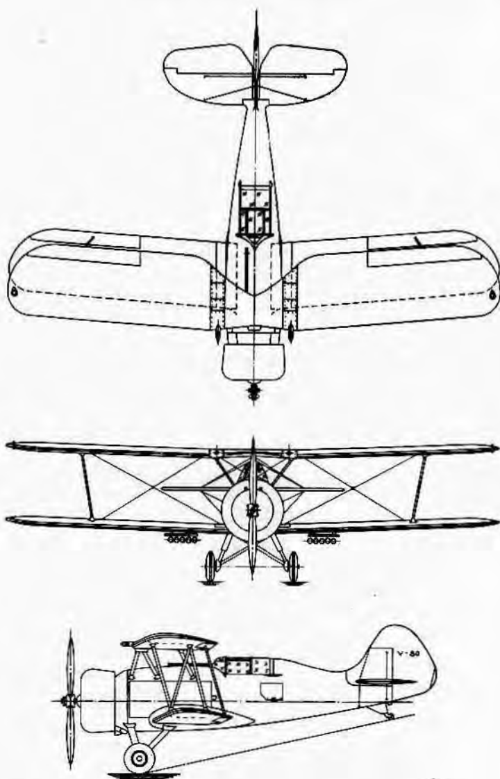
CHANCE VOGHT CORPORATION East Hartford, Conn. CORSAIR V-80 — 1 PLACE ENGINE: PRATT & WHITNEY HORNET
