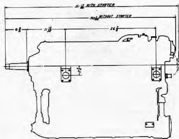
RANGER ENGINEERING CORPORATION Farmingdale, N. Y. MODEL 6-390 — 120 H.P. 6 CYLINDER INVERTED IN LINE AIRCOOLED
