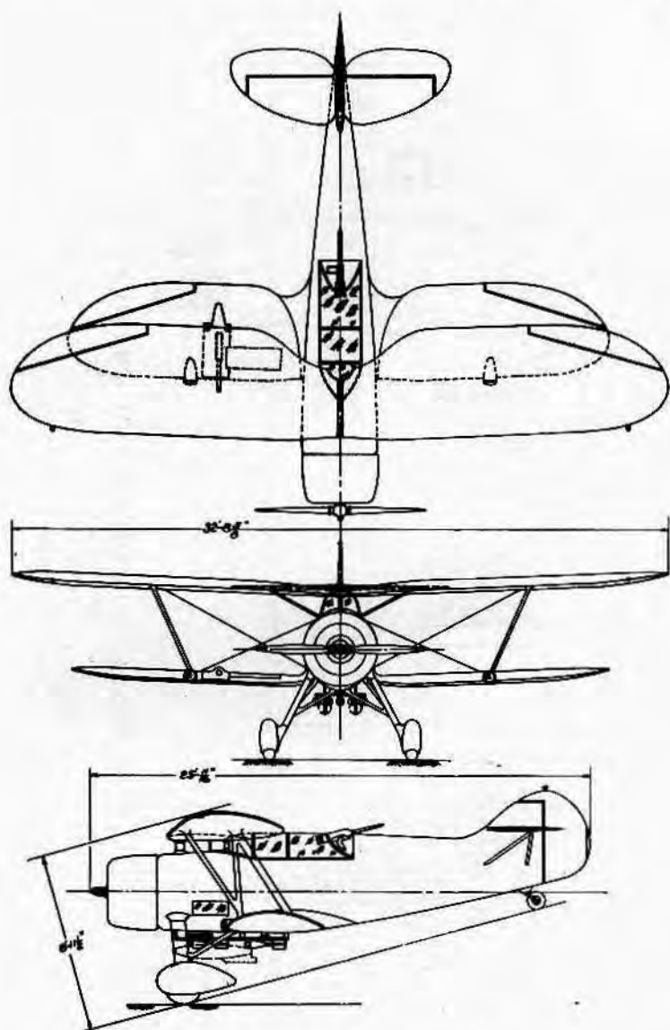
WACO AIRCRAFT COMPANY Troy, Ohio MODEL WHD-A — 2 PLACE ENGINE: WRIGHT WHIRLWIND
