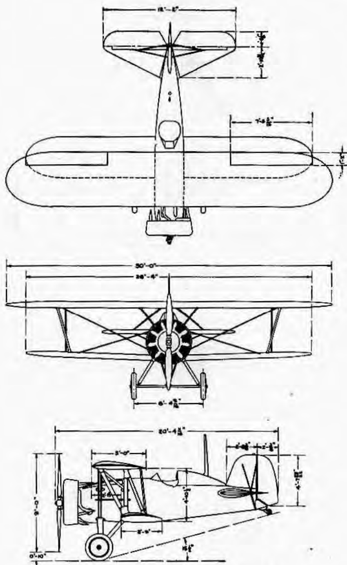
BOEING AIRCRAFT COMPANY Seattle, Wash. FIGHTER F4B-4 ENGINE: PRATT & WHITNEY WASP
