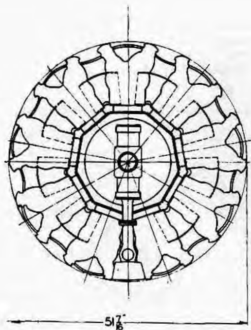
PRATT & WHITNEY AIRCRAFT COMPANY East Hartford, Conn. WASP H1 (GEARED 3:2 AND 4:3) — 500-550 H.P. 9 CYLINDER RADIAL AIRCOOLED
