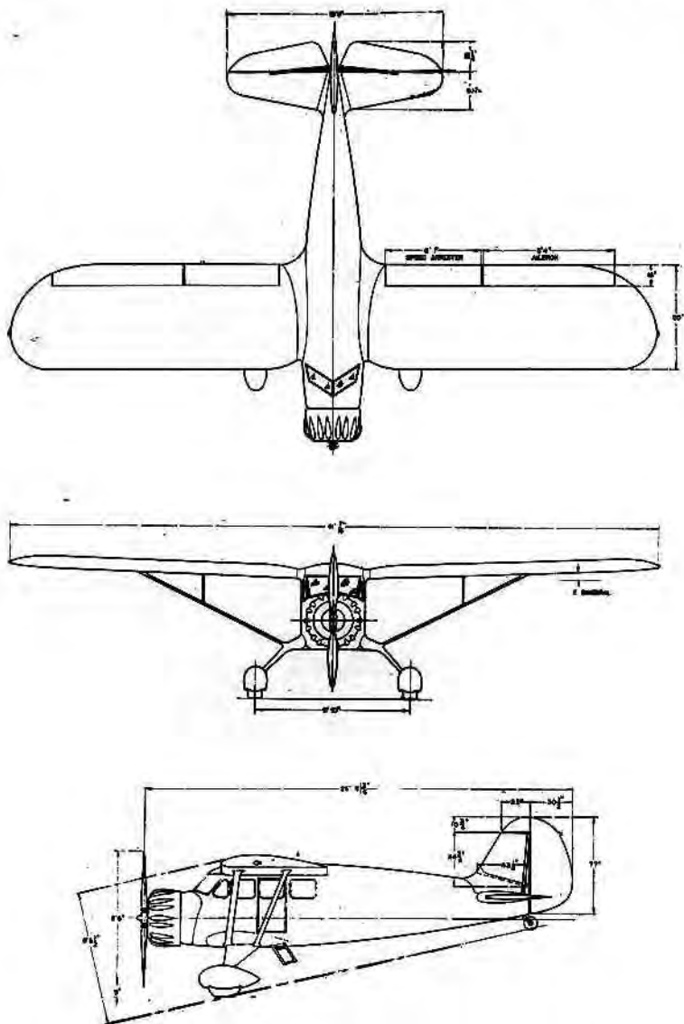
STINSON AIRCRAFT CORPORATION Wayne, Mich. RELIANT MODEL SR-5E — 4 PLACE ENGINE: LYCOMING
