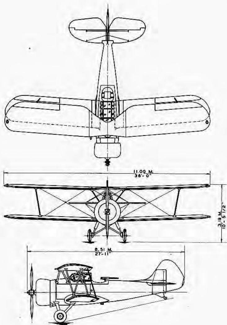
CHANCE VOUGHT CORPORATION East Hartford, Conn. CORSAIR SUPER V-90 — 2 PLACE ENGINE: PRATT & WHITNEY HORNET
