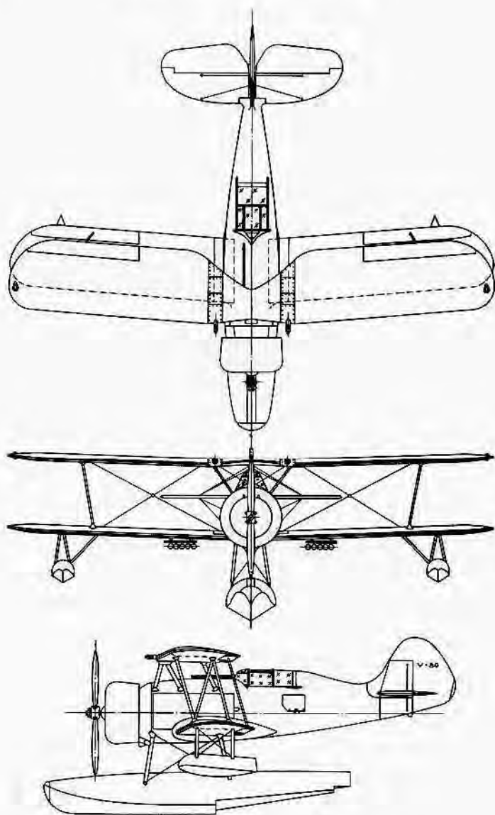
CHANCE VOUGHT CORPORATION East Hartford, Conn. CORSAIR V-80 SEAPLANE — 1 PLACE ENGINE: PRATT & WHITNEY HORNET
