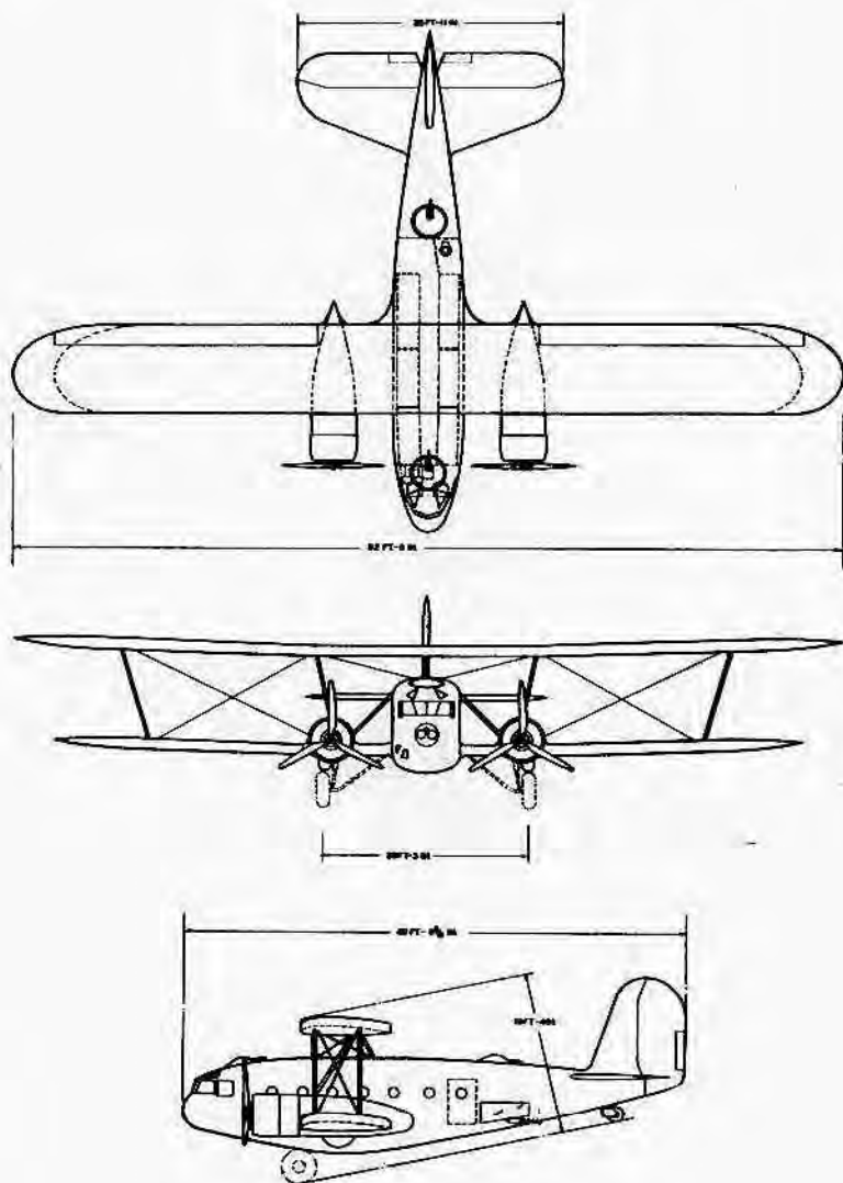
CURTISS-WRIGHT AIRPLANE COMPANY Robertson, Mo. CONDOR BOMBER BT-32 ENGINES: TWO WRIGHT CYCLONES 715 H.P.
