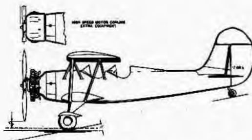
STINSON AIRCRAFT CORPORATION Wayne, Mich. SENIOR TRAINER — 2 PLACE ENGINE: LYCOMING
