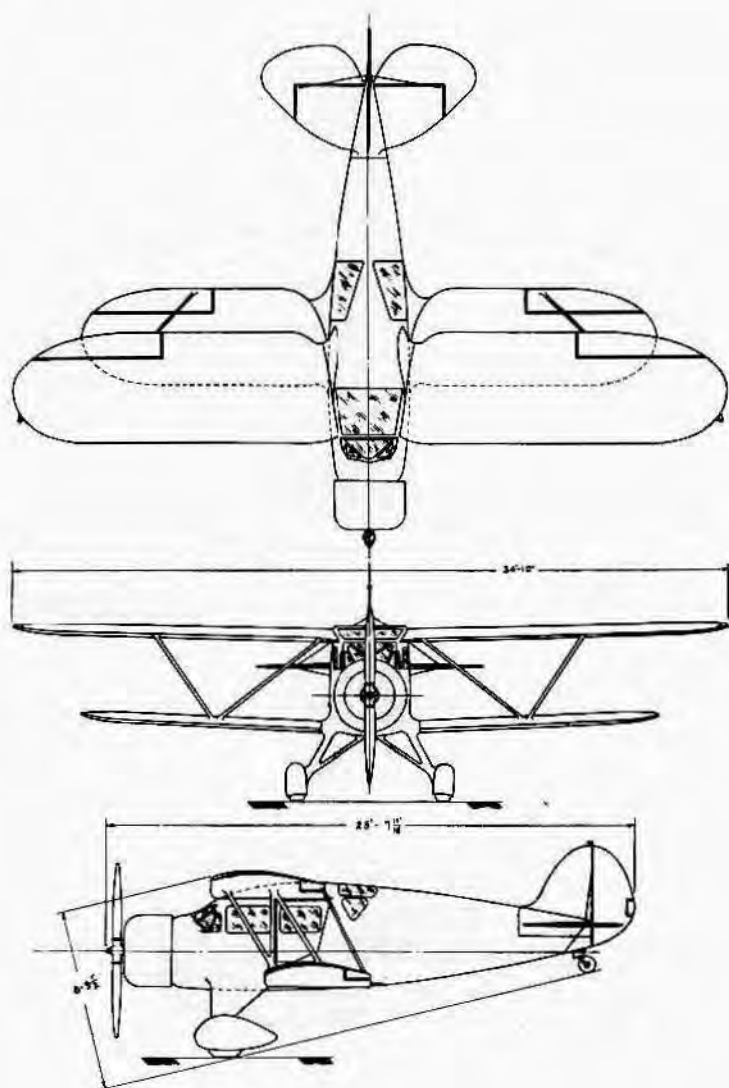
WACO AIRCRAFT COMPANY Troy, Ohio MODEL CJC — 4 PLACE ENGINE: WRIGHT WHIRLWIND
