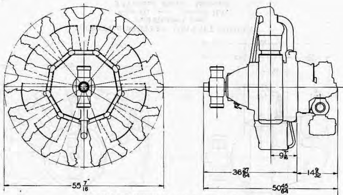
PRATT & WHITNEY AIRCRAFT COMPANY East Hartford, Conn. HORNET D1 (GEARED 3:2) — 650-700 H.P. 9 CYLINDER RADIAL AIRCOOLED
