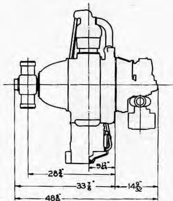
PRATT & WHITNEY AIRCRAFT COMPANY East Hartford, Conn. WASP H1 (GEARED 3:2 AND 4:3) — 500-550 H.P. 9 CYLINDER RADIAL AIRCOOLED
