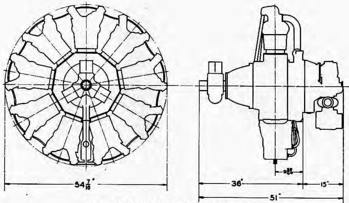
PRATT & WHITNEY AIRCRAFT COMPANY East Hartford, Conn. HORNET E (GEARED 3:2) — 675-750 H.P. 9 CYLINDER RADIAL AIRCOOLED
