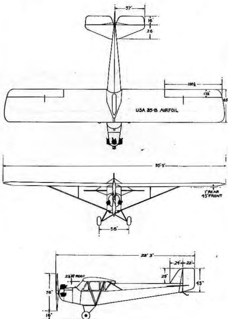
TAYLOR AIRCRAFT COMPANY Bradford, Pa. TAYLOR CUB F-2 — 2 PLACE ENGINE: AEROMARINE ARS-40
