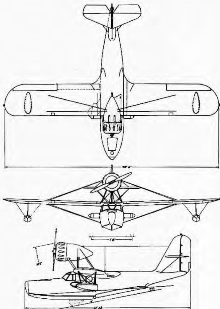
FLEETWINGS, INC. Bristol, Pa. MODEL F401 AMPHIBION — 4 PLACE ENGINE: JACOBS 225 H.P.
