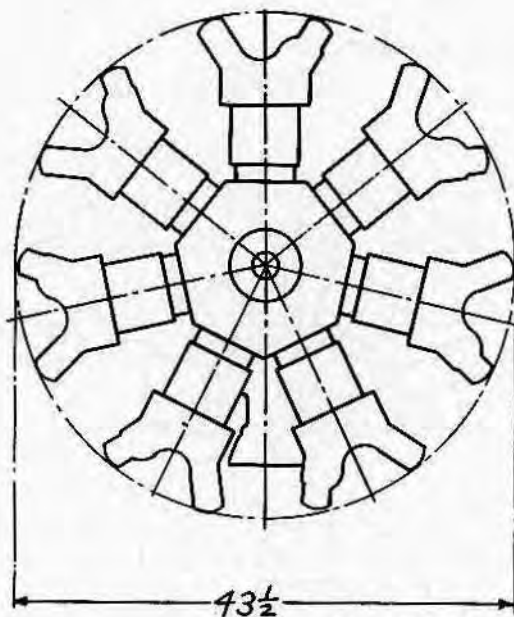
JACOBS AIRCRAFT ENGINE COMPANY Pottstown, Penna. JACOBS MODEL L-4M — 225 H.P. 7 CYLINDER RADIAL AIRCOOLED
