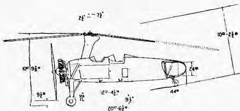
KELLETT AUTOGIRO CORPORATION Philadelphia, Pa. MODEL KD-1 — 2 PLACE ENGINE: JACOBS L-4
