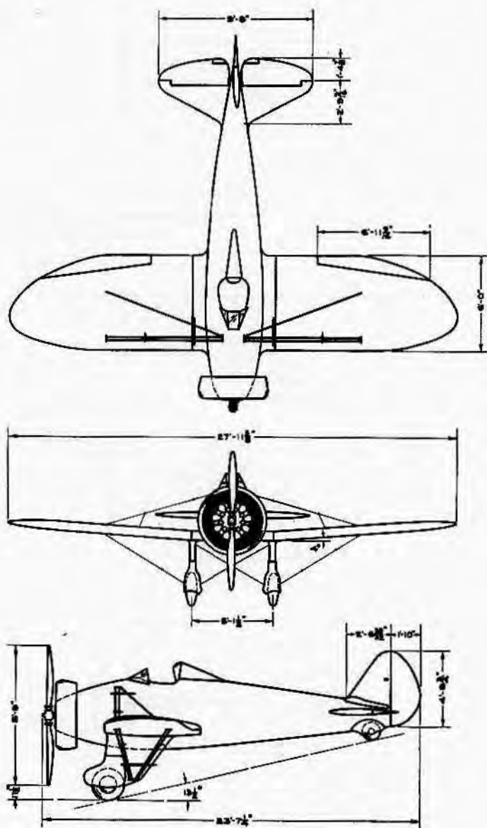
BOEING AIRCRAFT COMPANY Seattle, Wash. PURSUIT P-26A — MODEL 281 ENGINE: PRATT & WHITNEY WASP
