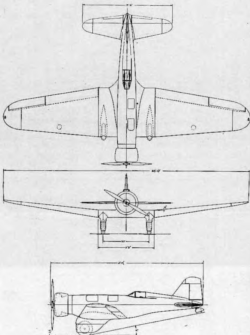
THE NORTHROP CORPORATION Inglewood, Calif. GAMMA — 1 PLACE ENGINE: PRATT & WHITNEY HORNET WRIGHT CYCLONE
