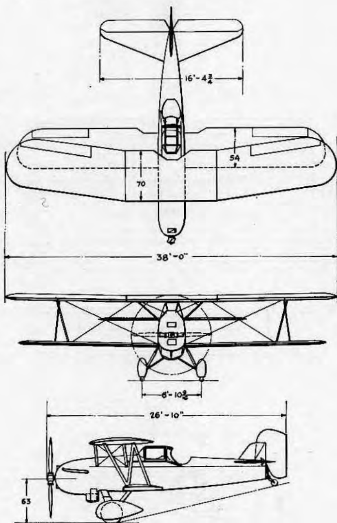
CURTISS AEROPLANE & MOTOR COMPANY Buffalo, N. Y. FALCON OBSERVATION O-39 ENGINE: CURTISS CONQUEROR 650 H.P.
