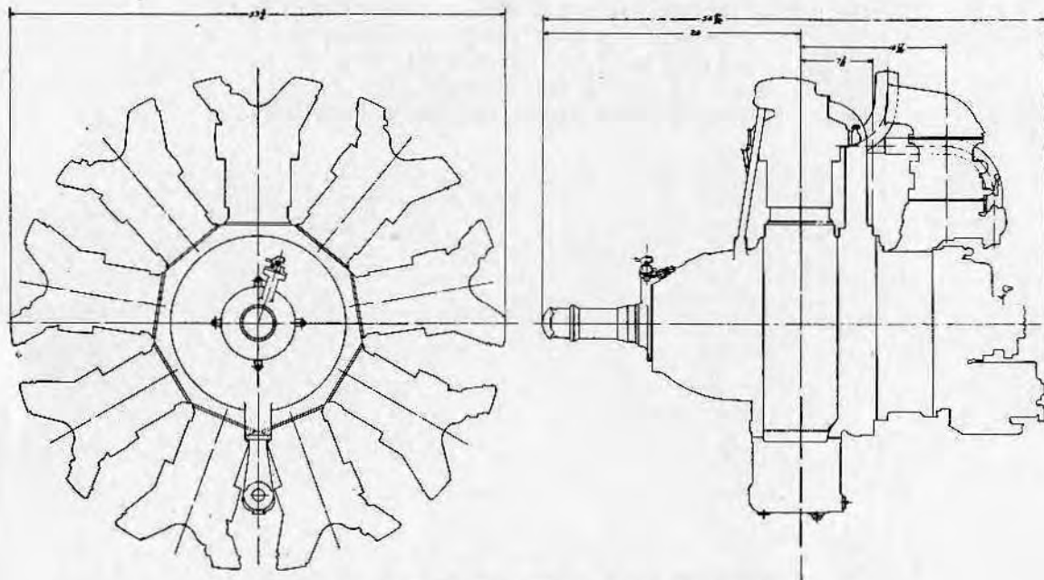
WRIGHT AERONAUTICAL CORPORATION Paterson, N. J. WRIGHT CYCLONE (GEARED 8:5) — 715 H.P. 9 CYLINDER FIXED RADIAL AIRCOOLED
