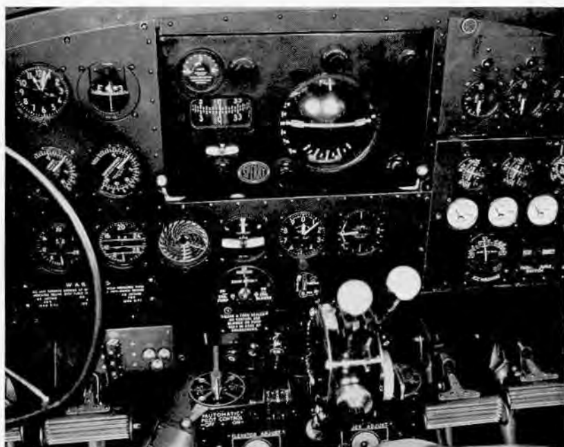
SPERRY AUTOMATIC PILOT
