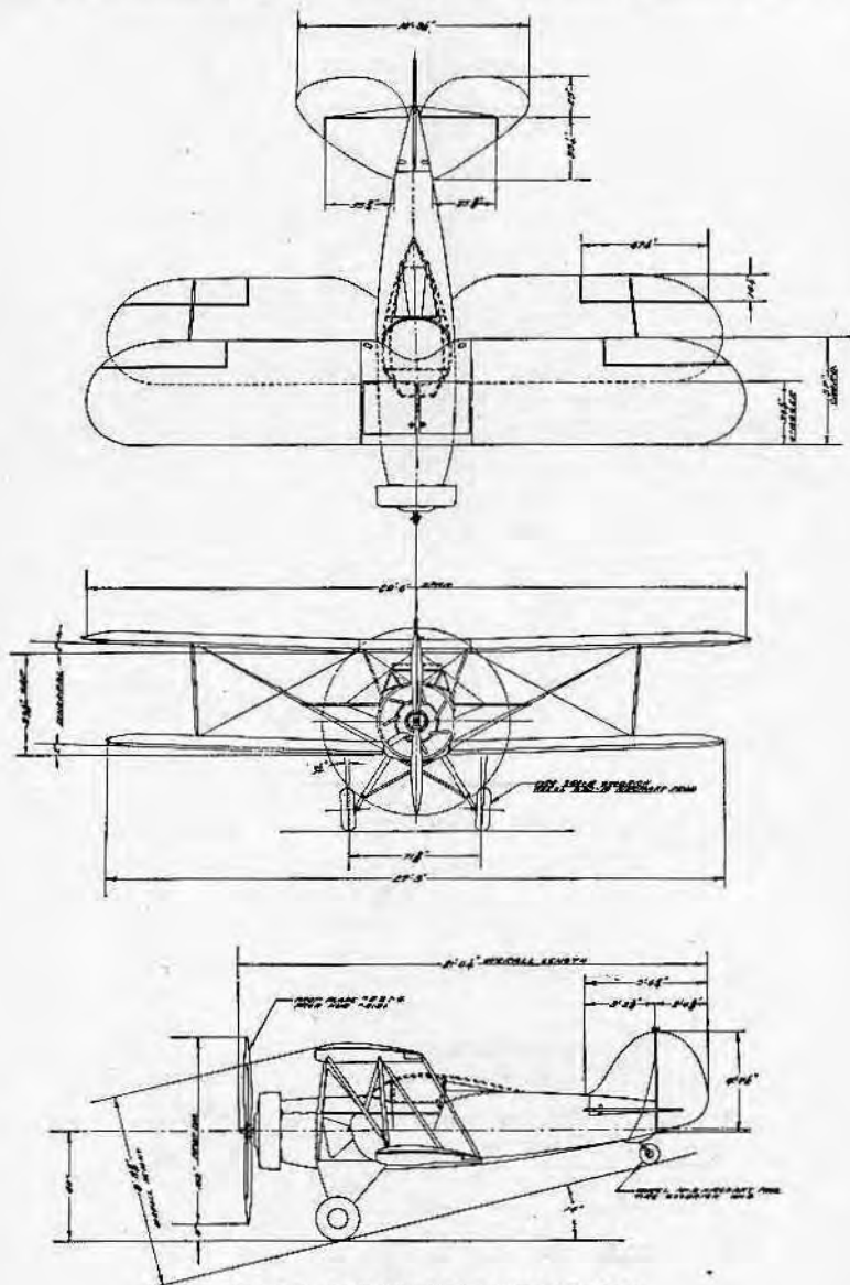
WACO AIRCRAFT COMPANY Troy, Ohio MODEL A — 2 PLACE ENGINE: CONTINENTAL JACOBS LA-1
