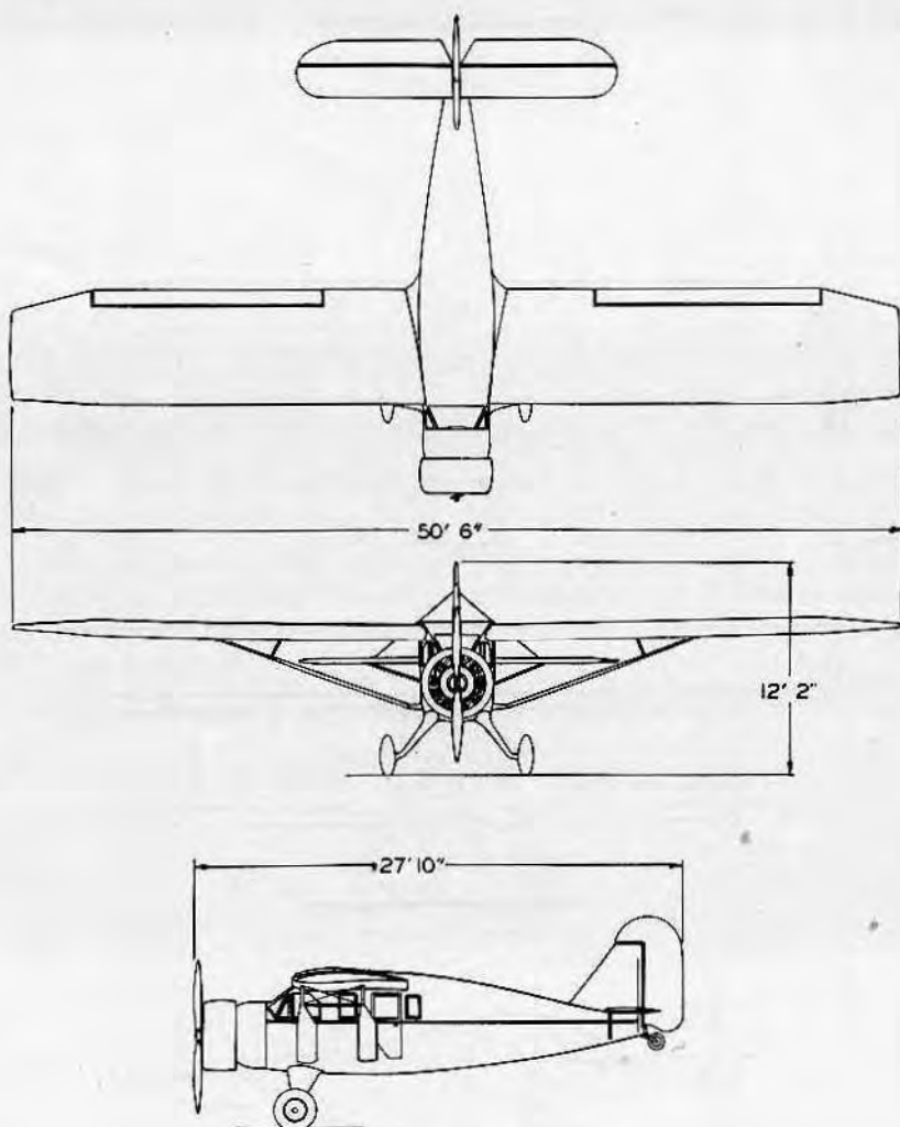
BELLANCA AIRCRAFT CORPORATION New Castle, Del. SENIOR PACEMAKER — 6 PLACE ENGINE: PRATT & WHITNEY WASP JUNIOR WRIGHT WHIRLWIND
