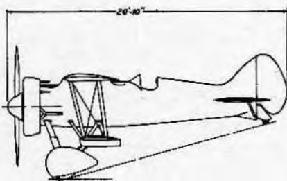
B/J AIRCRAFT CORPORATION Baltimore, Md. NAVY FIGHTER XF2J-1 — 2 PLACE ENGINE: WRIGHT WHIRLWIND
