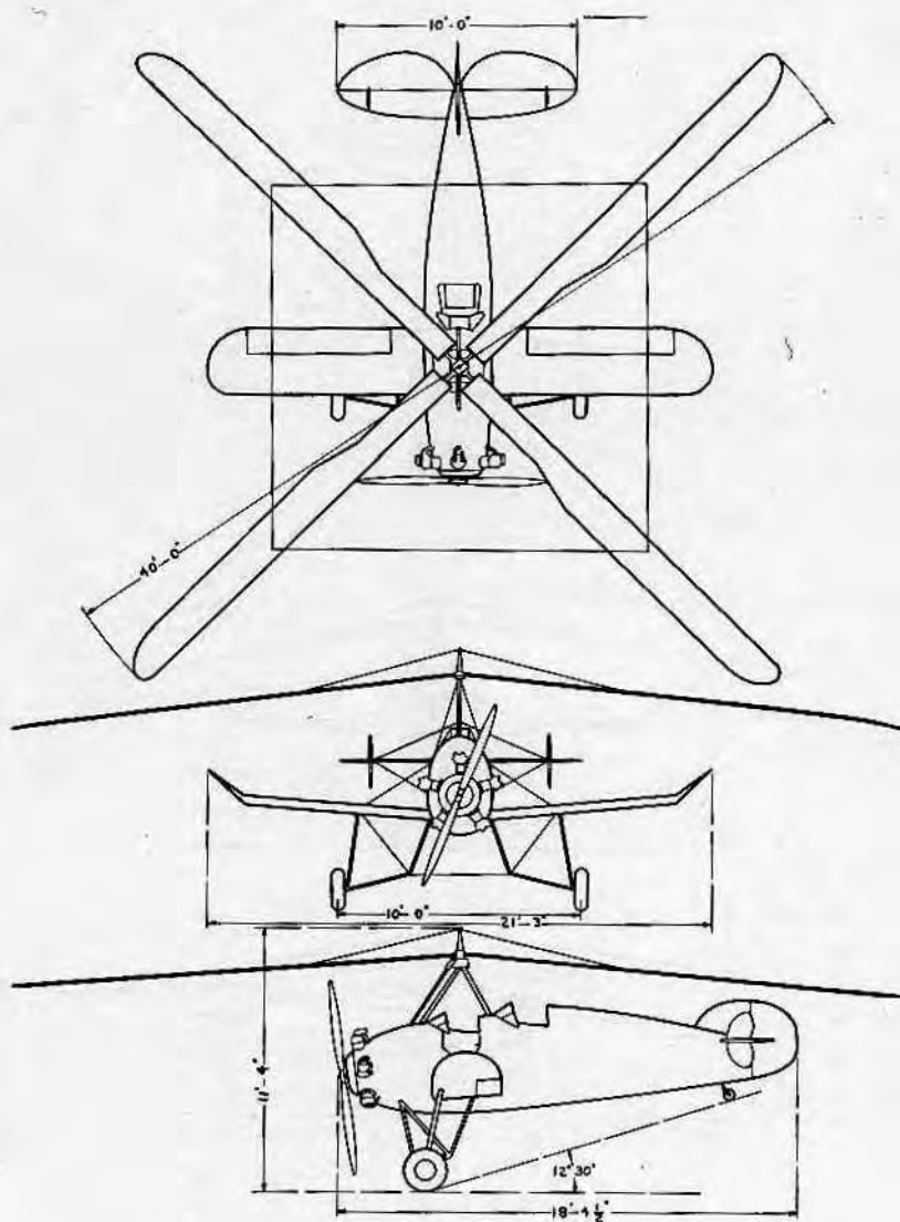
PITCAIRN AUTOGIRO COMPANY Willow Grove, Pa. MODEL PA-18 — 2 PLACE ENGINE: KINNER R-5
