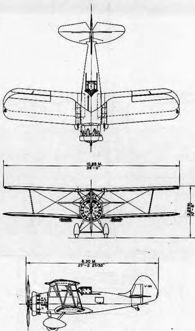
CHANCE VOGHT CORPORATION East Hartford, Conn. CORSAIR V-80 — 1 PLACE ENGINE: PRATT & WHITNEY HORNET
