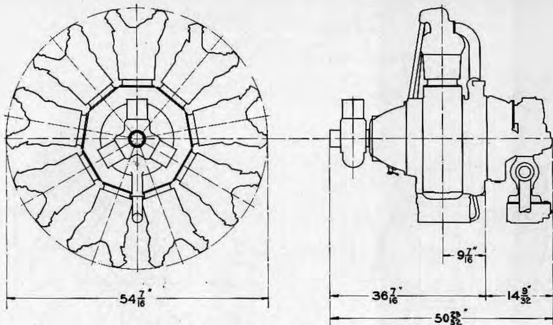
PRATT & WHITNEY AIRCRAFT COMPANY East Hartford, Conn. HORNET D (GEARED 3:2) — 700 H.P. 9 CYLINDER RADIAL AIRCOOLED
