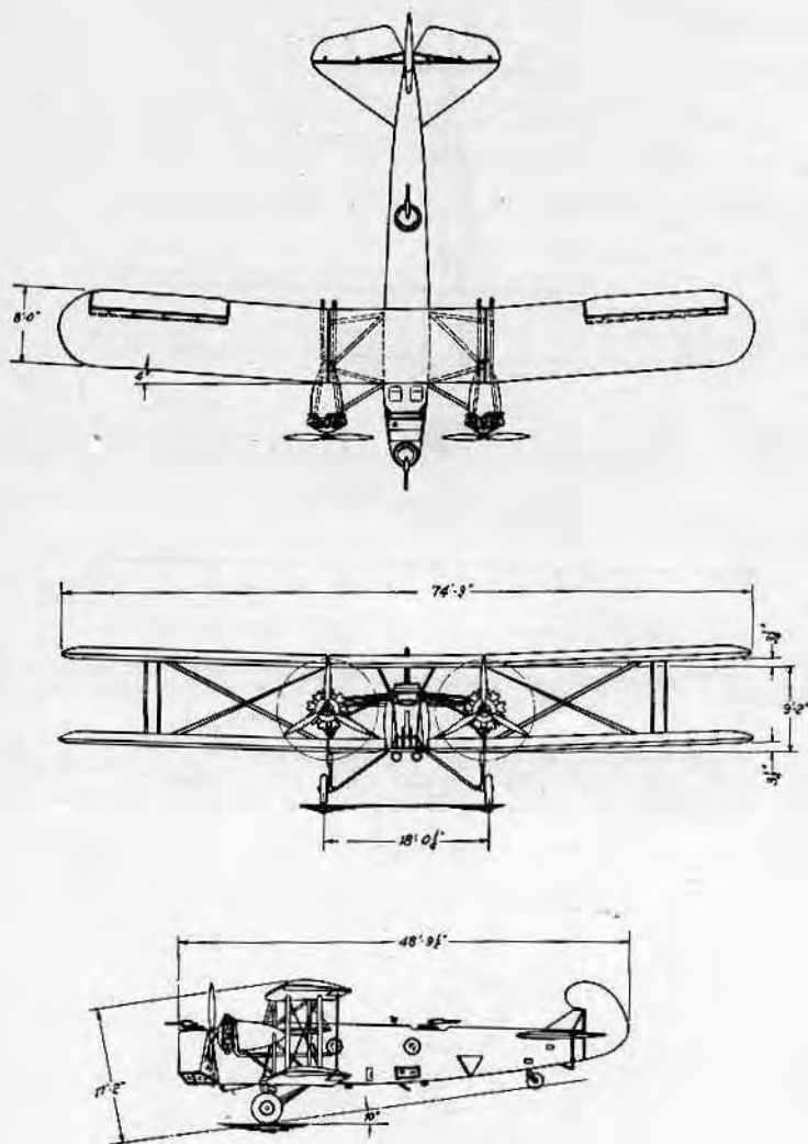
KEYSTONE AIRCRAFT CORPORATION Bristol, Pa. BOMBARDMENT B6-A ENGINES: TWO WRIGHT CYCLONES
