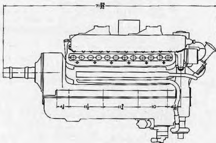
WRIGHT AERONAUTICAL CORPORATION Paterson, N. J. CURTISS CONQUEROR (GEARED) — 650 H.P. 12 CYLINDER V TYPE LIQUID COOLED
