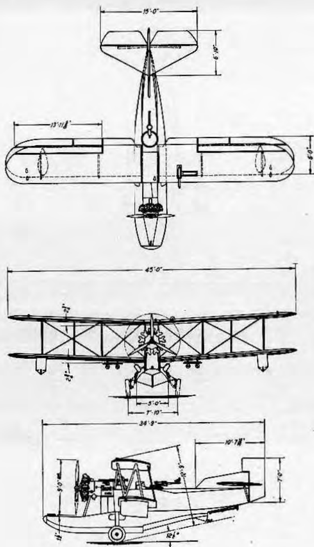
KEYSTONE AIRCRAFT CORPORATION Bristol, Pa. MODEL OL9 ENGINE: PRATT & WHITNEY WASP
