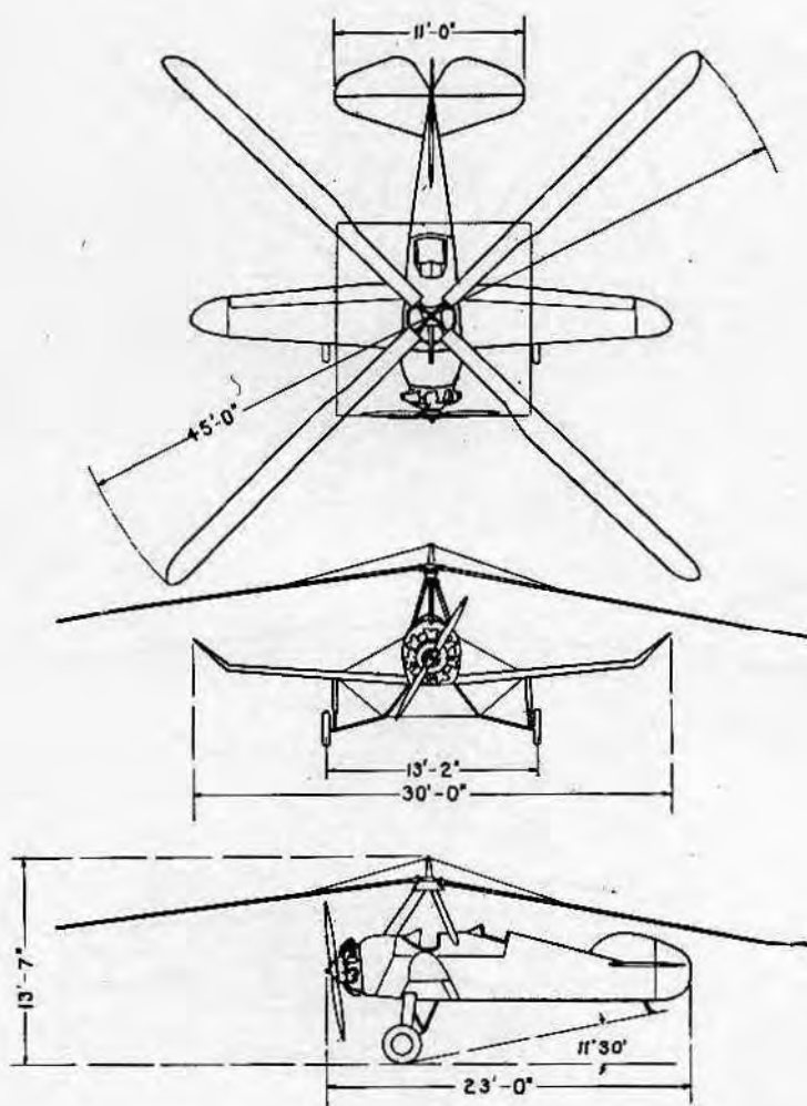
PITCAIRN AUTOGIRO COMPANY Willow Grove, Pa. MODEL PCA-2; PCA-3 — 3 PLACE ENGINE: PRATT & WHITNEY WASP JUNIOR WRIGHT WHIRLWIND 300
