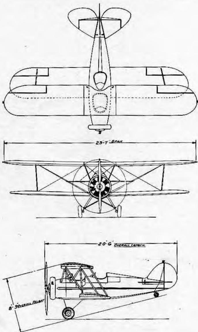
WACO AIRCRAFT COMPANY Troy, Ohio MODELS PBF & UBF — 3 PLACE ENGINE: JACOBS LA-1 CONTINENTAL R-670
