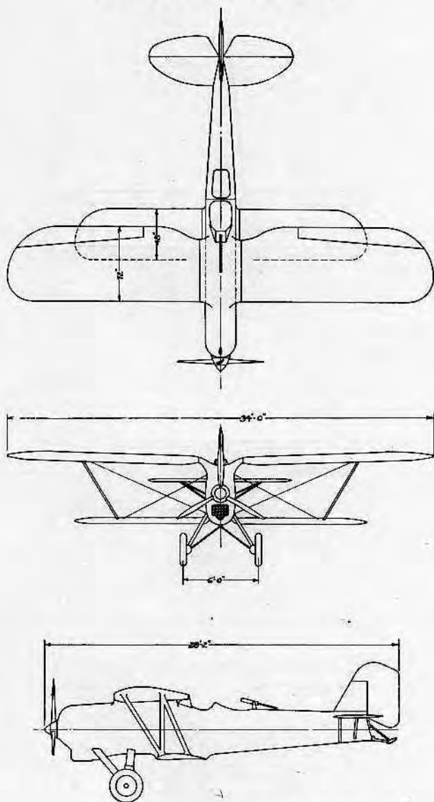
B/J AIRCRAFT CORPORATION Baltimore, Md. ARMY PURSUIT Y1P-16 — 2 PLACE ENGINE: CURTISS CONQUEROR
