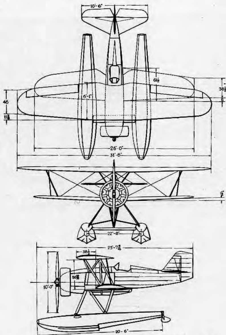
CURTISS AEROPLANE & MOTOR COMPANY Buffalo, N. Y. HAWK PURSUIT SEAPLANE ENGINE: WRIGHT CYCLONE F — 700 H.P.
