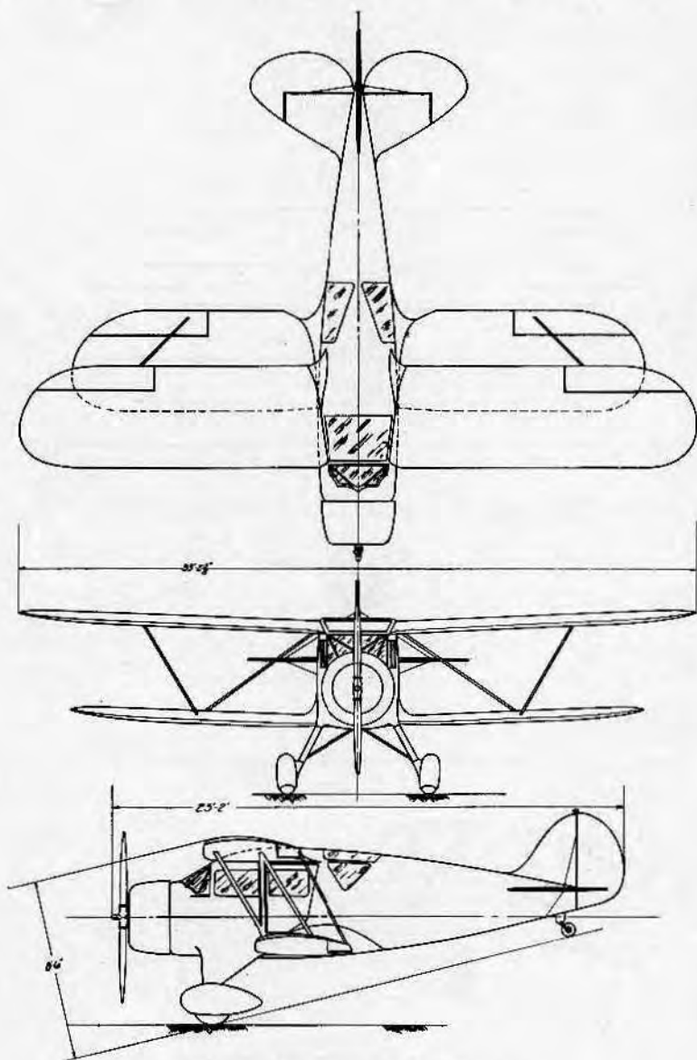
WACO AIRCRAFT COMPANY Troy, Ohio MODEL UIC — 4 PLACE ENGINE: CONTINENTAL R-670
