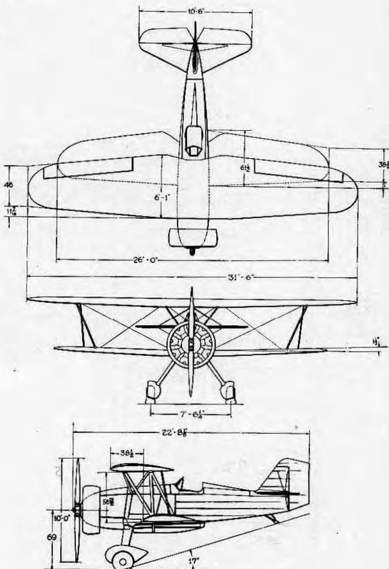
CURTISS AEROPLANE & MOTOR COMPANY Buffalo, N. Y. HAWK PURSUIT LAND PLANE ENGINE: WRIGHT CYLCONE F — 700 H.P.
