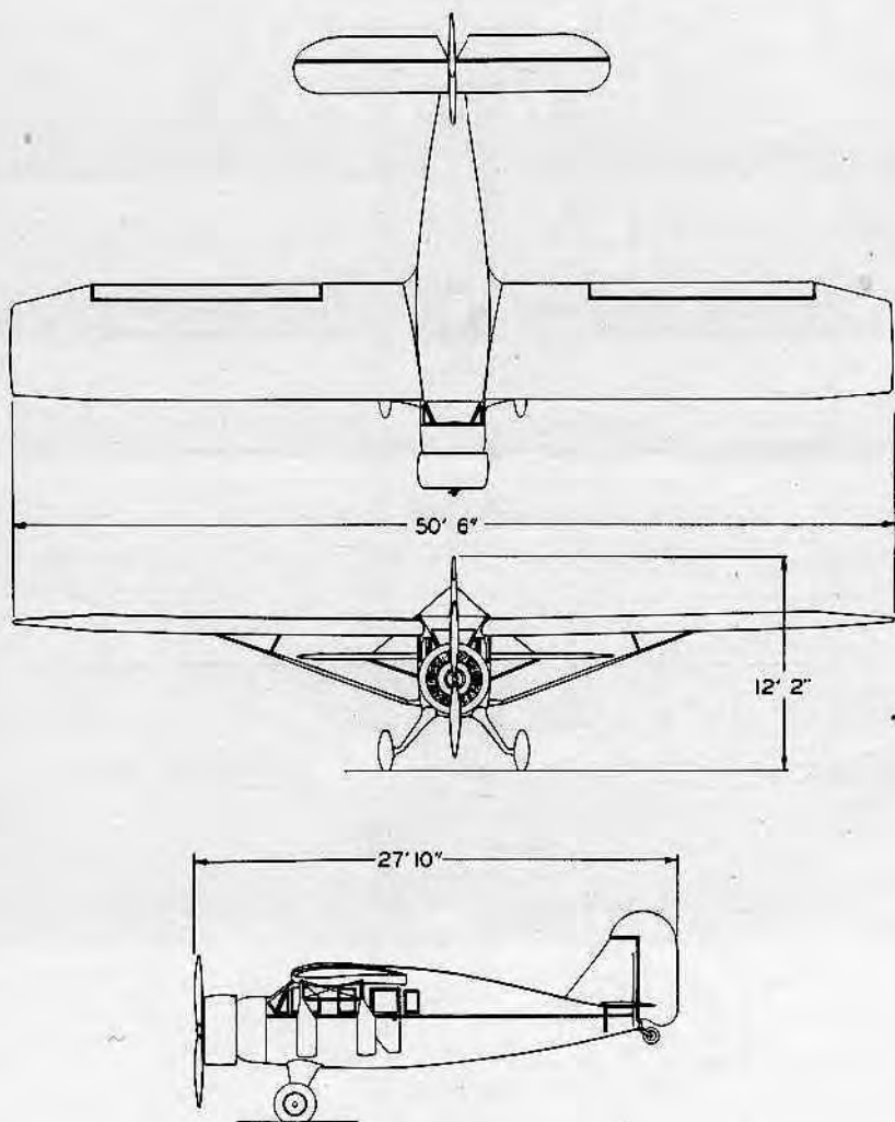
BELLANCA AIRCRAFT CORPORATION - New Castle, Del. SENIOR SKYROCKET — 6-8 PLACE SENIOR SKYROCKET STANDARD SENIOR SKYROCKET DeLuxe ENGINE: PRATT & WHITNEY WASP
