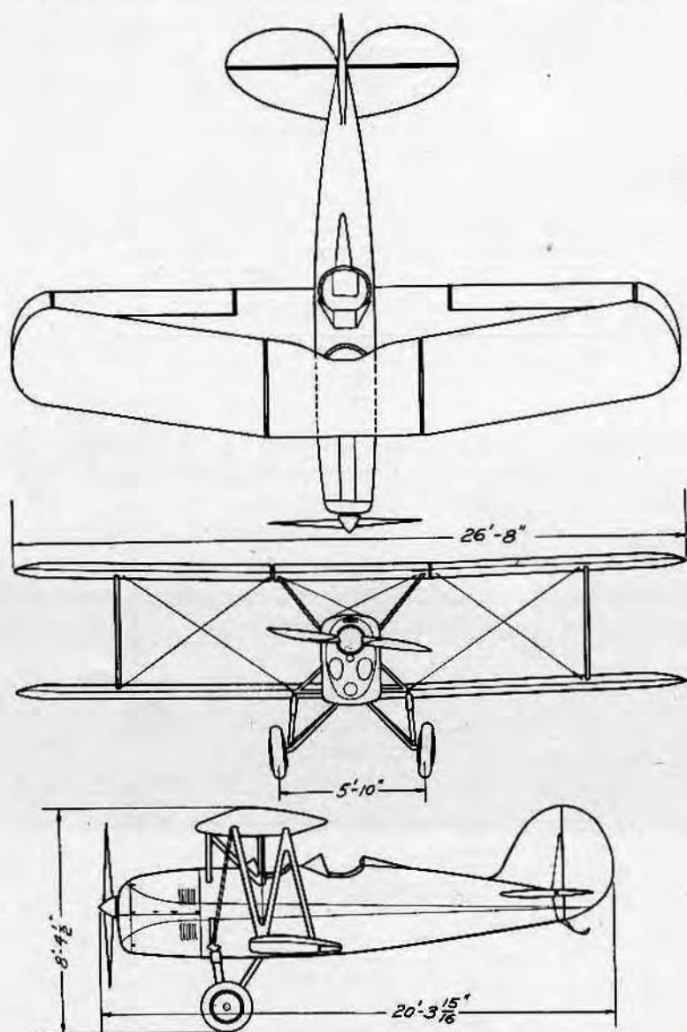
GREAT LAKES AIRCRAFT CORPORATION Cleveland, Ohio MODEL 2T-1E — 2 PLACE ENGINE: HI-DRIVE AMERICAN CIRRUS
