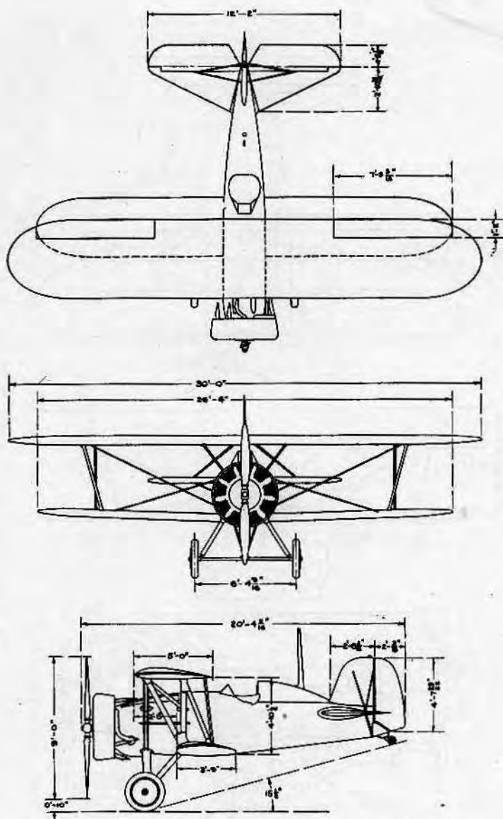
BOEING AIRPLANE COMPANY Seattle, Wash. FIGHTER F4B-4 ENGINE: PRATT & WHITNEY WASP
