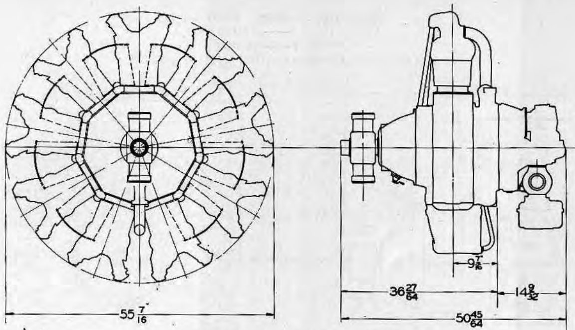
PRATT & WHITNEY AIRCRAFT COMPANY East Hartford, Conn. HORNET D1 (GEARED 3:2) — 575-700 H.P. 9 CYLINDER RADIAL AIRCOOLED
