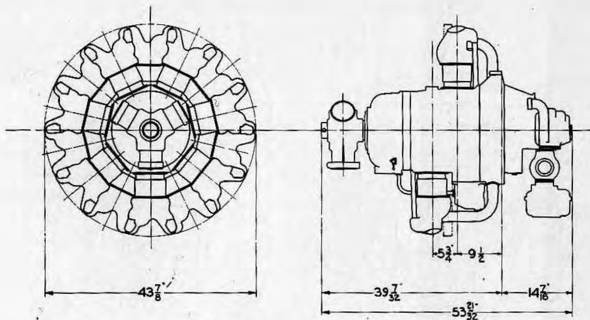
PRATT & WHITNEY AIRCRAFT COMPANY East Hartford, Conn. TWIN WASP JUNIOR (GEARED 3:2 AND 4:3) — 650-700 H.P. 14 CYLINDER RADIAL AIRCOOLED
