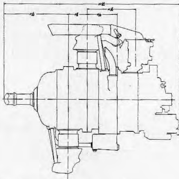
WRIGHT AERONAUTICAL CORPORATION Paterson, N. J. WRIGHT DOUBLE ROW WHIRLWIND — 700 H.P. 14 CYLINDER 2 ROW FIXED RADIAL AIRCOOLED
