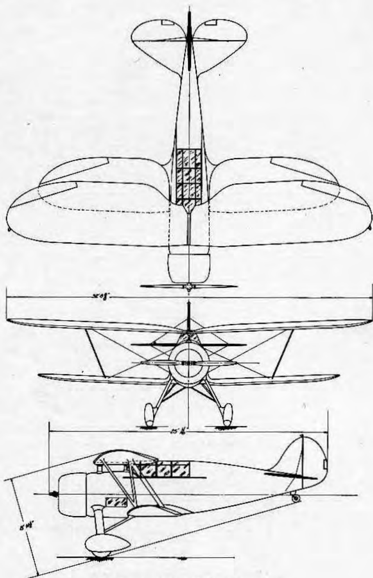
WACO AIRCRAFT COMPANY Troy, Ohio MODEL WHD — 2 PLACE ENGINE: WRIGHT WHIRLWIND
