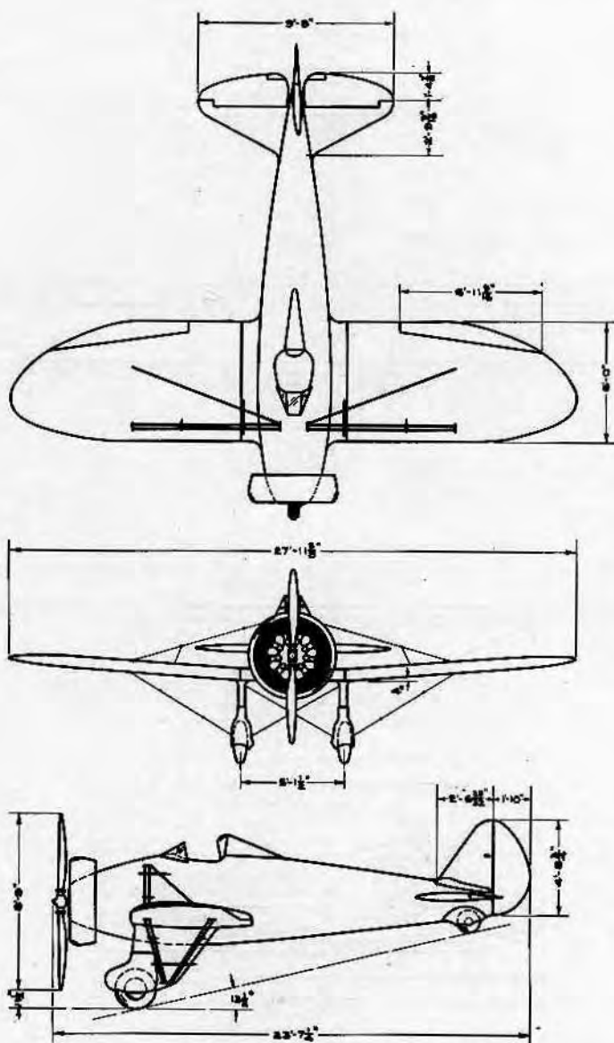
BOEING AIRPLANE COMPANY Seattle, Wash. PURSUIT P-26A ENGINE: PRATT & WHITNEY WASP
