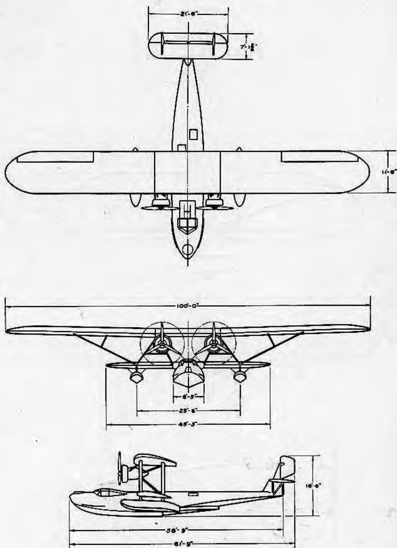
CONSOLIDATED AIRCRAFT CORPORATION Buffalo, N. Y. PATROL FLYING BOAT P2Y-1 ENGINES: TWO GEARED WRIGHT CYCLONES
