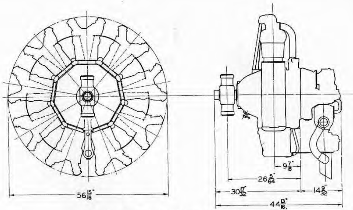
PRATT & WHITNEY AIRCRAFT COMPANY East Hartford, Conn. HORNET B1 — 575-625 H.P. 9 CYLINDER RADIAL AIRCOOLED
