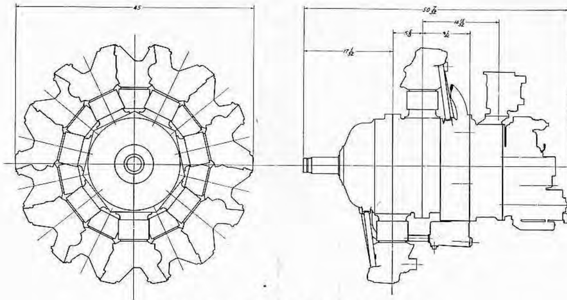
WRIGHT AERONAUTICAL CORPORATION Paterson, N. J. Two Row Whirlwind — 625 H.P. 14 CYLINDER RADIAL AIRCOOLED
