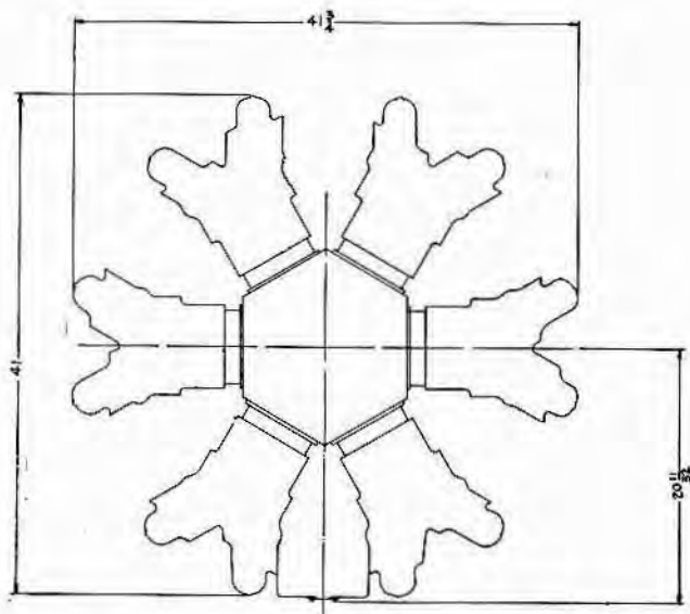
WRIGHT AERONAUTICAL CORPORATION Paterson, N. J. CURTISS CHALLENGER — 185 H.P. 6 CYLINDER RADIAL AIRCOOLED
