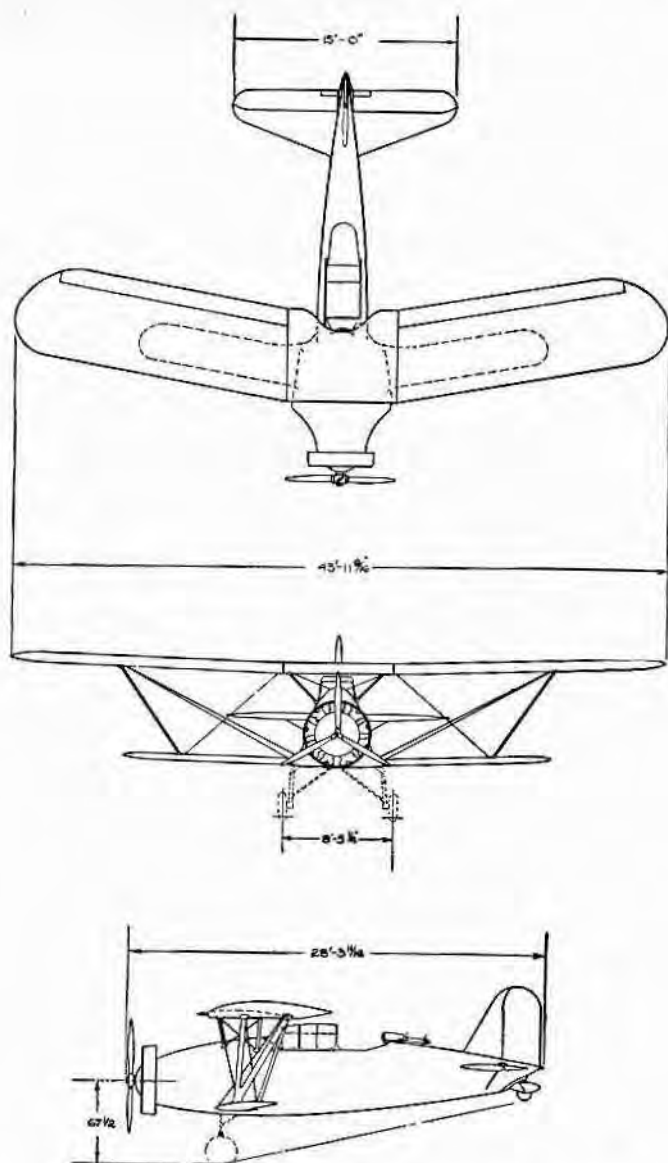
CURTISS AEROPLANE & MOTOR COMPANY Buffalo, N. Y. OBSERVATION YO-40 — "RAVEN" ENGINE: WRIGHT CYCLONE
