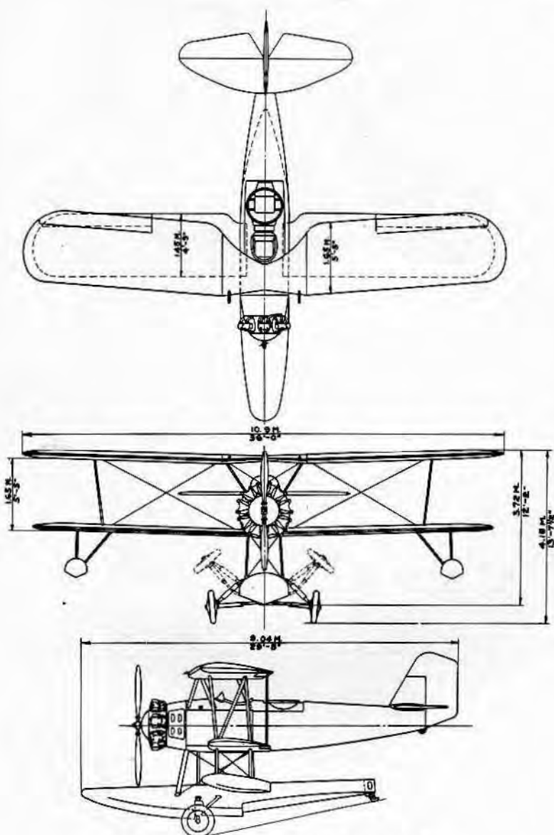
CHANCE VUGHT CORPORATION East Hartford, Conn. OBSERVATION O2U-4 ENGINE: PRATT & WHITNEY WASP
