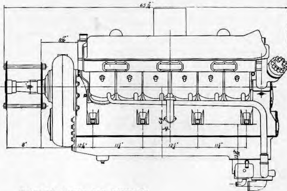
PACKARD MOTOR CAR COMPANY Detroit, Mich. MODEL 2A-1500 (GEARED) — 600 H.P. 12 CYLINDER V TYPE WATERCOOLED
