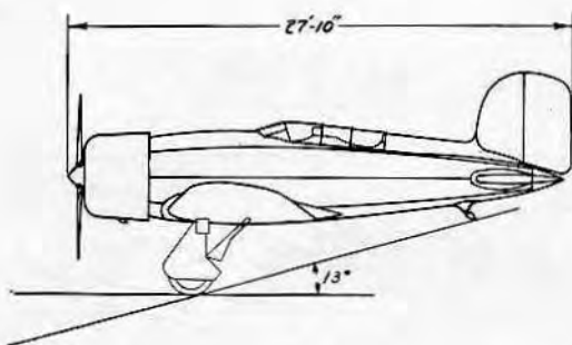
DETROIT AIRCRAFT CORPORATION Detroit, Mich. DETROIT LOCKHEED ALTAIR — 2 PLACE ENGINE: PRATT & WHITNEY WASP WRIGHT CYCLONE
