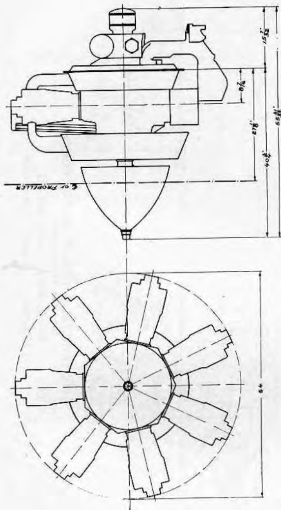
E. W. BLISS COMPANY Brooklyn, N. Y. BLISS-NEPTUNE — 400 H.P. 7 CYLINDER RADIAL AIRCOOLED
