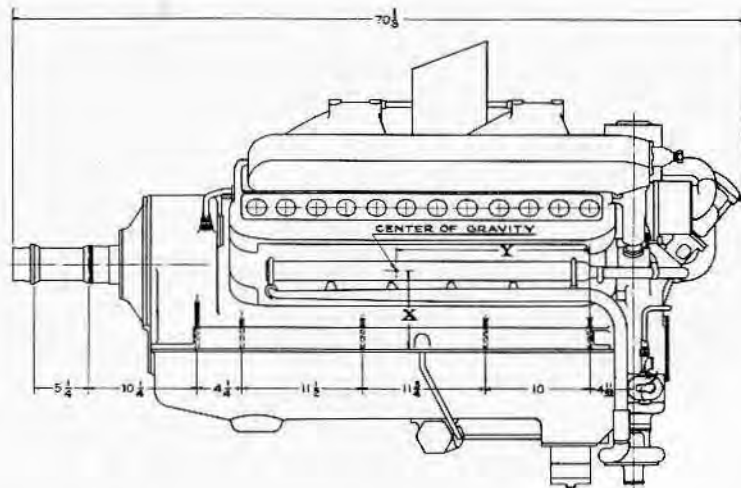
WRIGHT AERONAUTICAL CORPORATION Paterson, N. J. CURTISS CONQUEROR (GEARED) — 600 H.P. 12 CYLINDER V TYPE LIQUIDCOOLED
