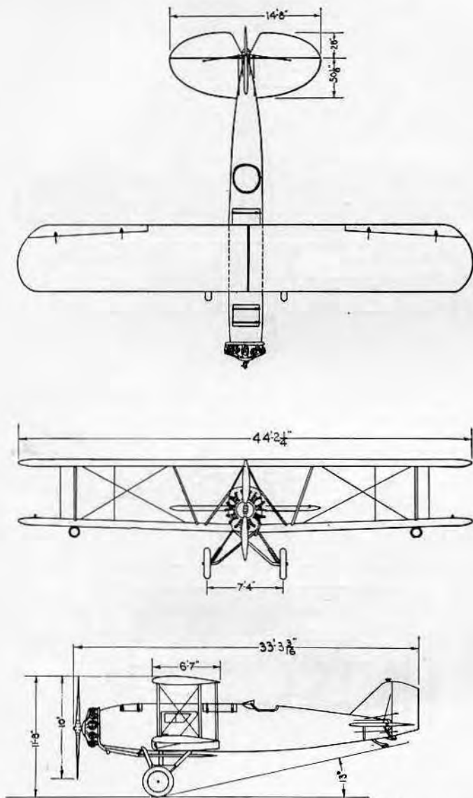
BOEING AIRPLANE COMPANY Seattle, Wash. MODEL 40 B-4 — 5 PLACE ENGINE: PRATT & WHITNEY HORNER
