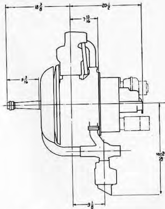
CONTINENTAL AIRCRAFT ENGINE COMPANY Detroit, Mich. MODEL A70 165 H.P. 7 CYLINDER RADIAL AIRCOOLED
