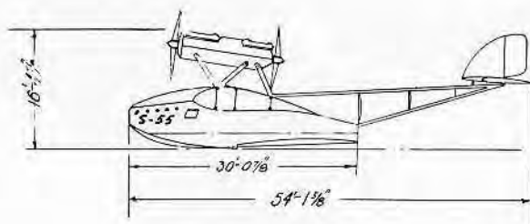
AMERICAN AERONAUTICAL CORPORATION New York City AMERICAN MARCHETTI S-55 16 PLACE ENGINE: TWO ISOTTA FRASCHINI
