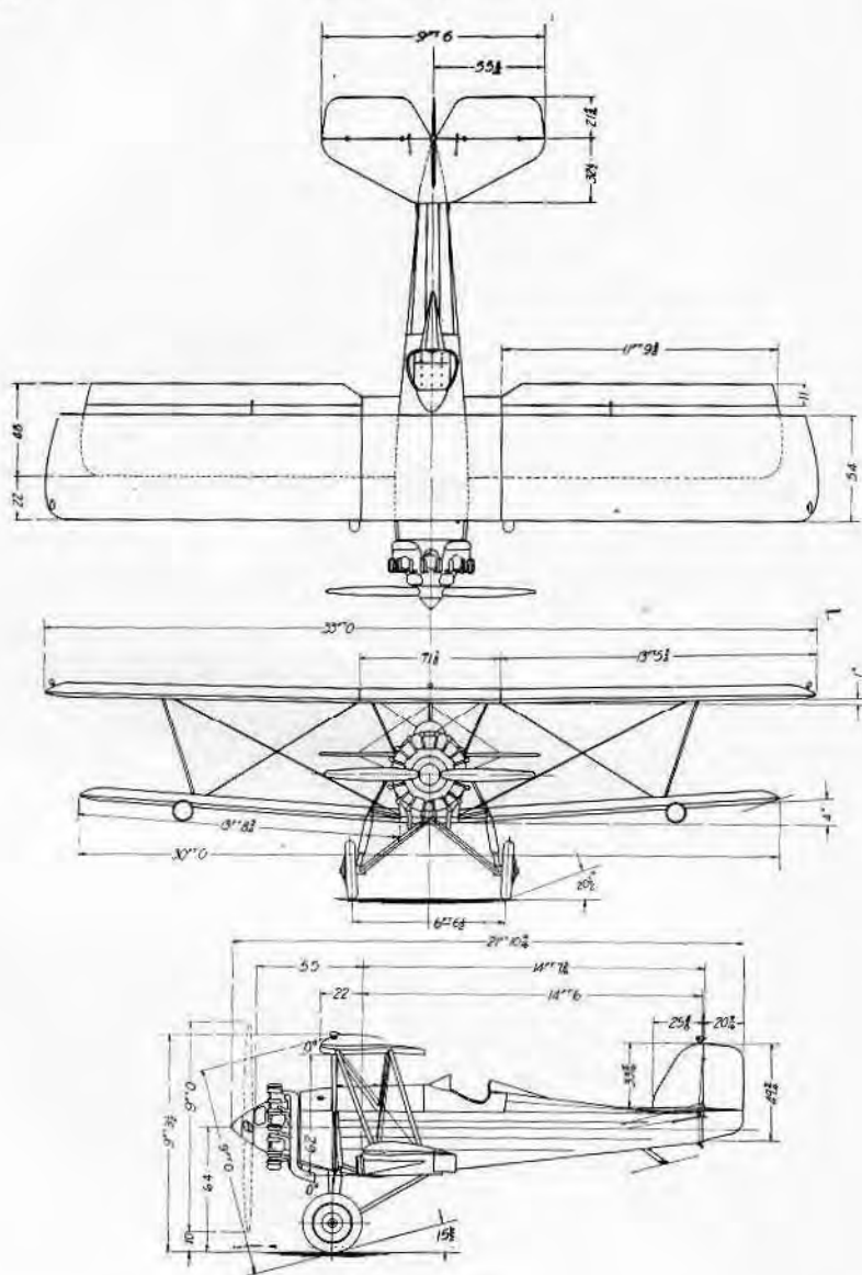
PITCAIRN AIRCRAFT, INC. Philadelphia, Pa. MAILWING 1 PLACE ENGINE: WRIGHT J-5
