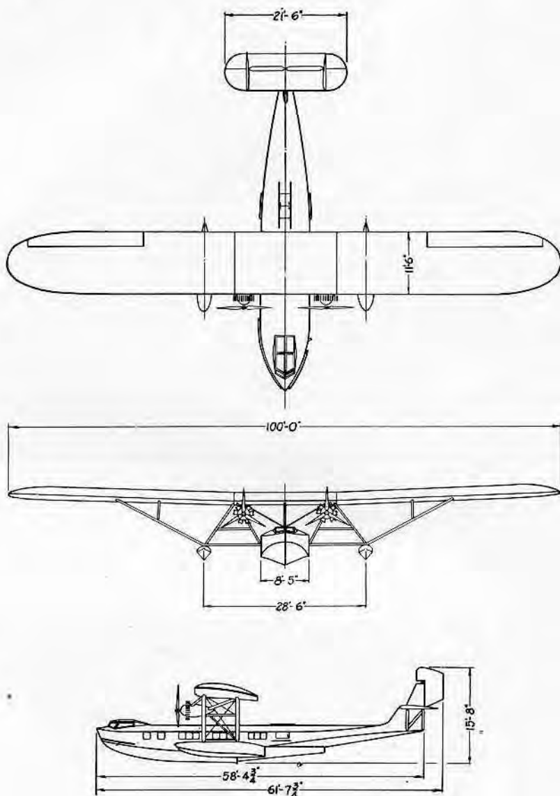
CONSOLIDATED AIRCRAFT CORPORATION Buffalo, N. Y. COMMODORE 22 PLACE ENGINE: TWO PRATT & WHITNEY HORNETS
