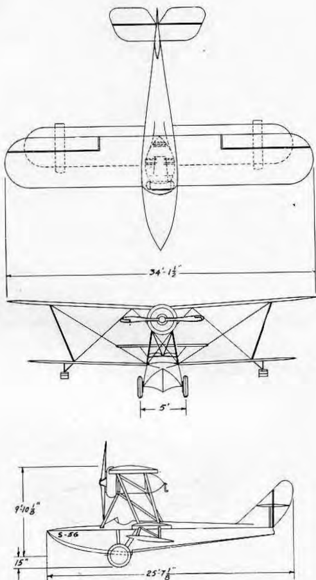
AMERICAN AERONAUTICAL CORPORATION New York City AMERICAN MARCHETTI S 56 3 PLACE ENGINE: KINNER
