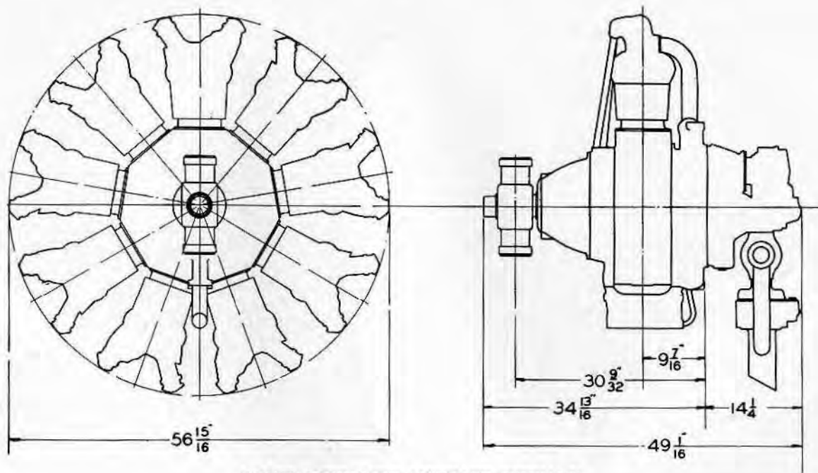
PRATT & WHITNEY AIRCRAFT COMPANY Hartford, Conn. HORNET B (GEARED) 550 H.P. 9 CYLINDER RADIAL AIRCOOLED
