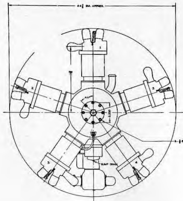
KINNER AIRPLANE & MOTOR CORPORATION Glendale, Calif. MODEL K5 100 H.P. 5 CYLINDER RADIAL AIRCOOLED
