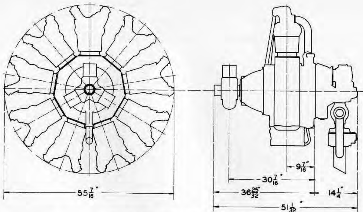
PRATT & WHITNEY AIRCRAFT COMPANY Hartford, Conn. HORNET (GEARED) 525 H.P. 9 CYLINDER RADIAL AIRCOOLED
