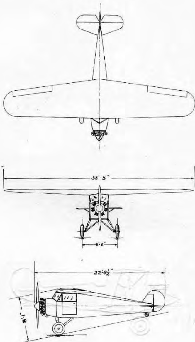
HUNTINGTON AIRCRAFT CORPORATION Bridgeport, Conn. MODEL 11 2 PLACE ENGINE: WARNER SCARAB
