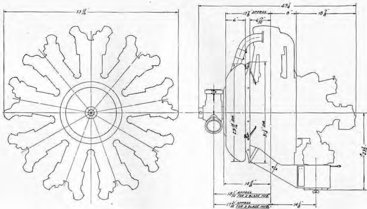
WRIGHT AERONAUTICAL CORPORATION Paterson, N. J. CYCLONE 525 H.P. 9 CYLINDER RADIAL AIRCOOLED
