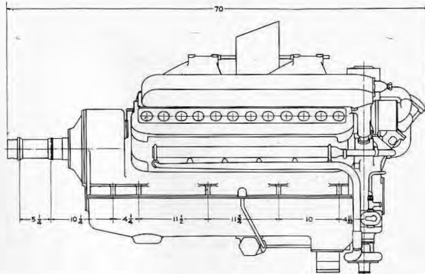
CURTISS AEROPLANE & MOTOR COMPANY, INC. Buffalo, N. Y. CONQUEROR (GEARED) 600 H.P. 12 CYLINDER V TYPE WATERCOOLED
