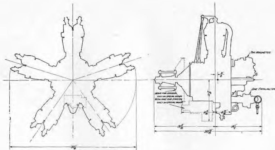
SIEMENS & HALSKE American Representative: K. G. FRANK 75 West Street, New York City MODEL SH 13 80 H.P. 5 CYLINDER RADIAL AIRCOOLED
