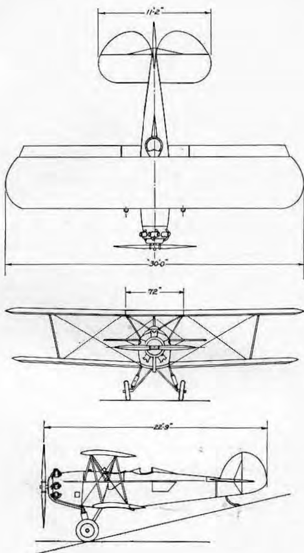
FAIRCHILD AVIATION CORPORATION (KREIDER-REISNER DIVISION) Hagerstown, Md. MODEL KR 34 3 PLACE ENGINE: WRIGHT WHIRLWIND 165
