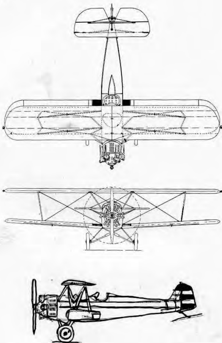
COMMAND-AIRE, INC. Little Rock, Ark. MODEL 5C3 3 PLACE ENGINE: CURTISS CHALLENGER
